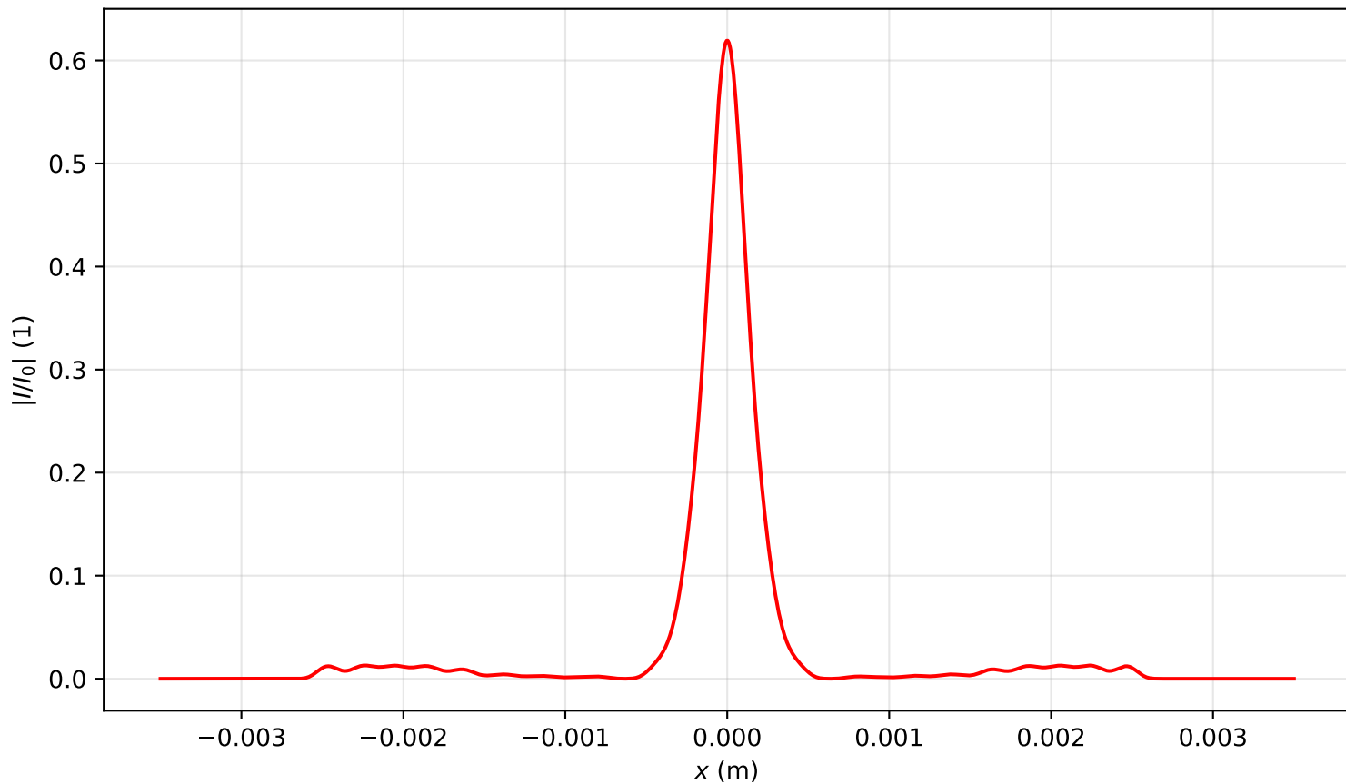
Intensity profile I(x, y = 0, z = 1.592)/I_0 , P_{in}=6.0P_{cr} , artificial time
